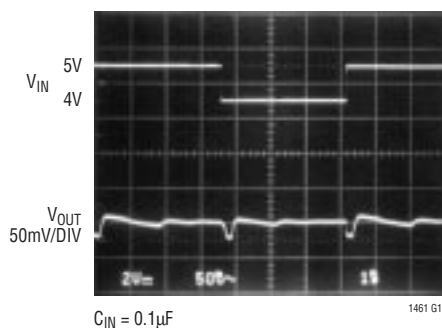
2.5V Line Transient Response
