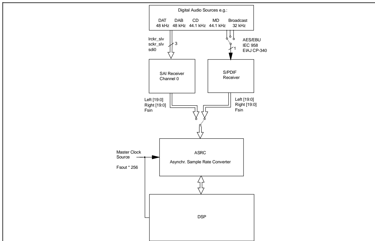
Figure 18. System Overview
