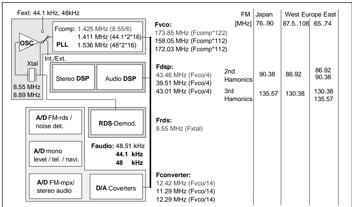
Figure 21. Clock Scheme
