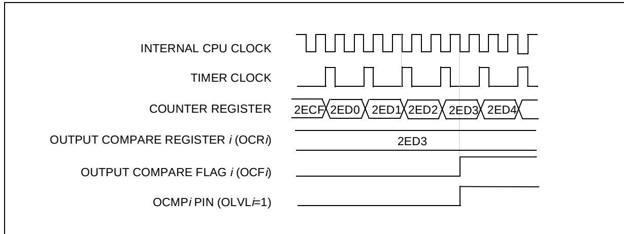
Figure 28. Output Compare Timing Diagram, f_{\text{TIMER}} = f_{\text{CPU}}/2
