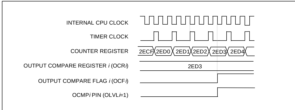
Figure 30. Output Compare Timing Diagram, f_{\text{TIMER}} = f_{\text{CPU}}/2
