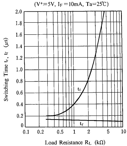
Switching Time vs. Resistance
