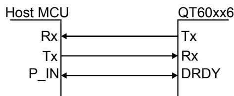
Figure 3-5 UART Connections
