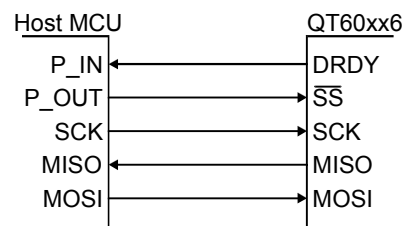
Figure 3-1 Basic SPI Connections
