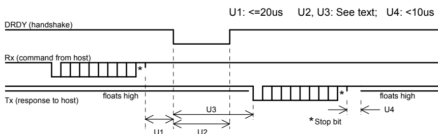
Figure 3-4 UART Timing
