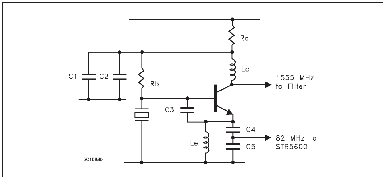
Fig. 6 Reference Oscillator
