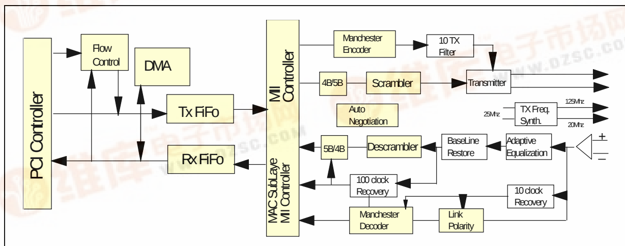
Figure 1. STE10/100Block Diagram
