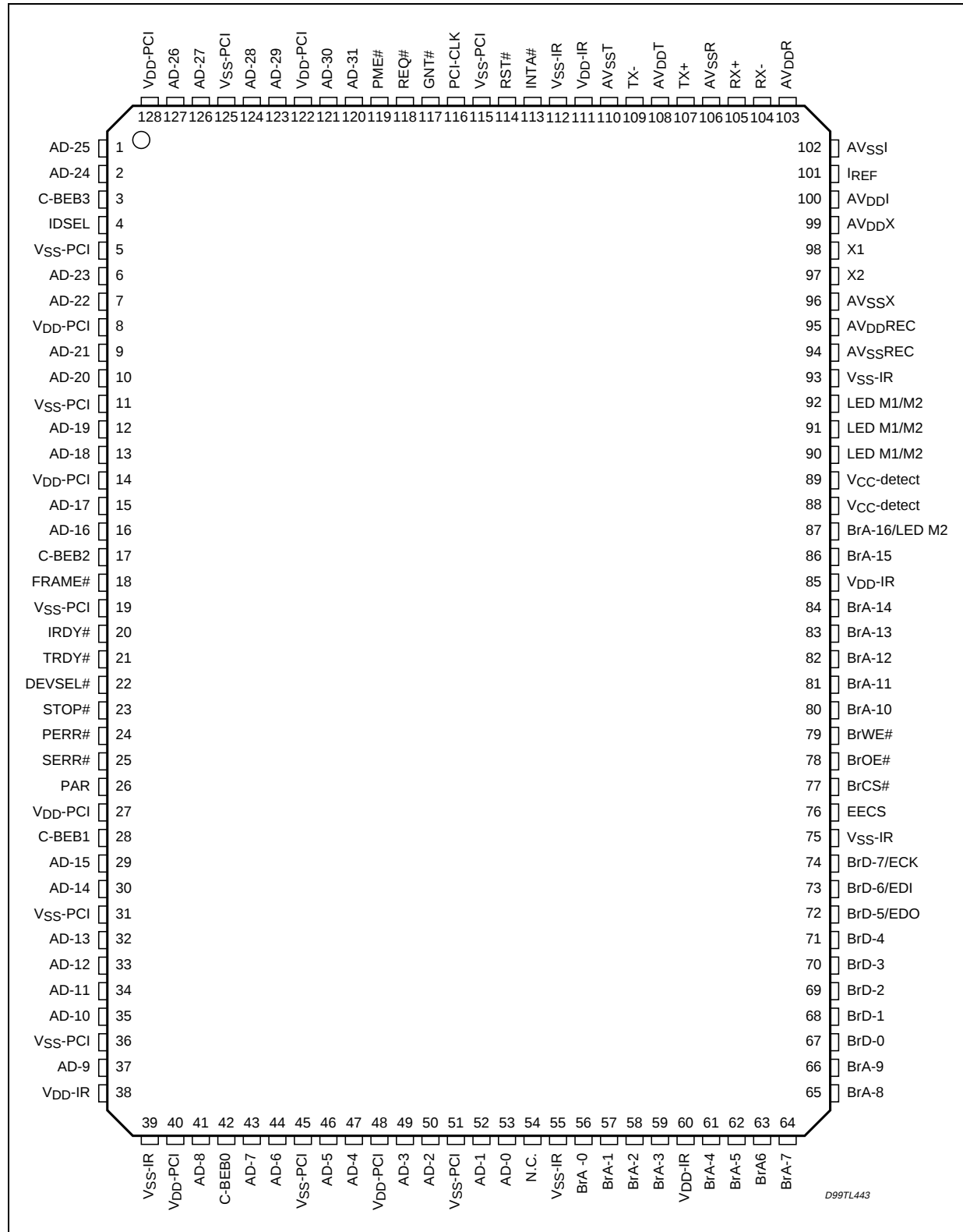
Figure 3. Pin Connection
