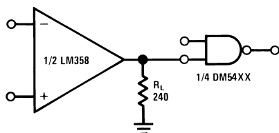
Driving TTL
