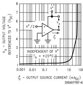
Output Characteristics Current Sourcing
