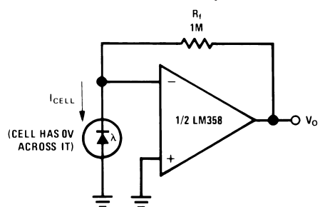
Photo Voltaic-Cell Amplifier
