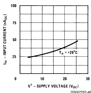
Input Current (LM2902 only)
