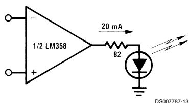
LED Driver
