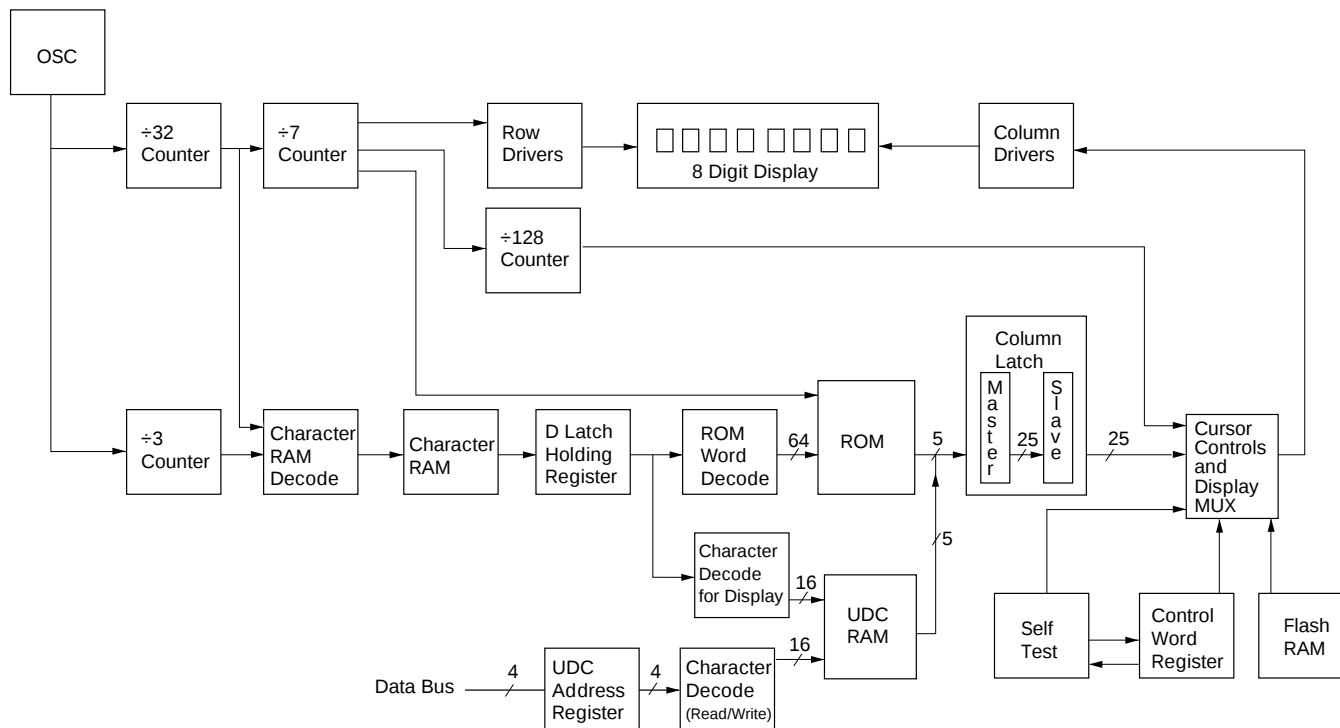
Figure 7. Block diagram
