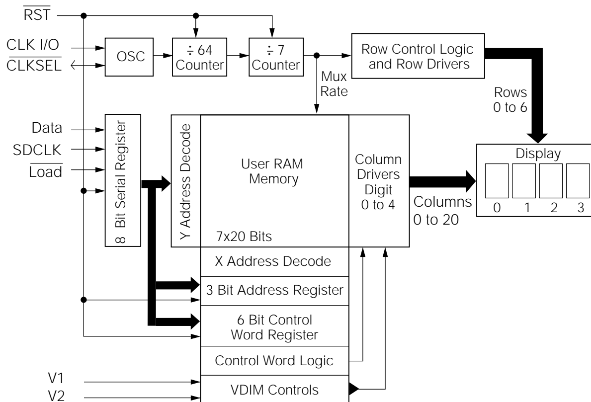
Figure 6. Block Diagram
