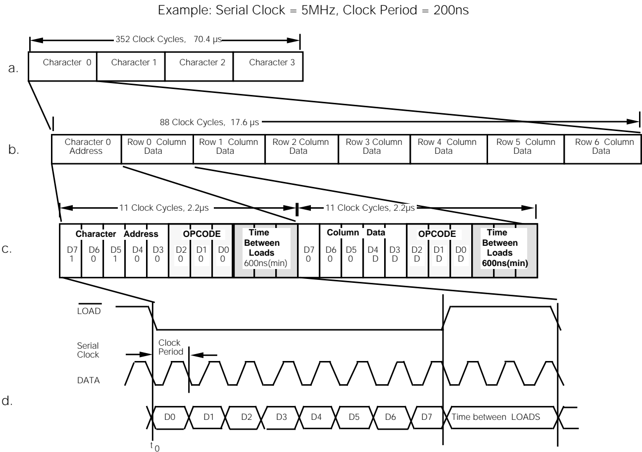
Figure 7a–d. Loading Serial Character Data
