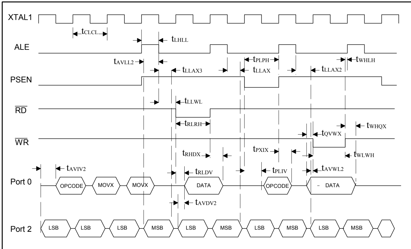
Figure 2. Page-Mode 1 Timing
