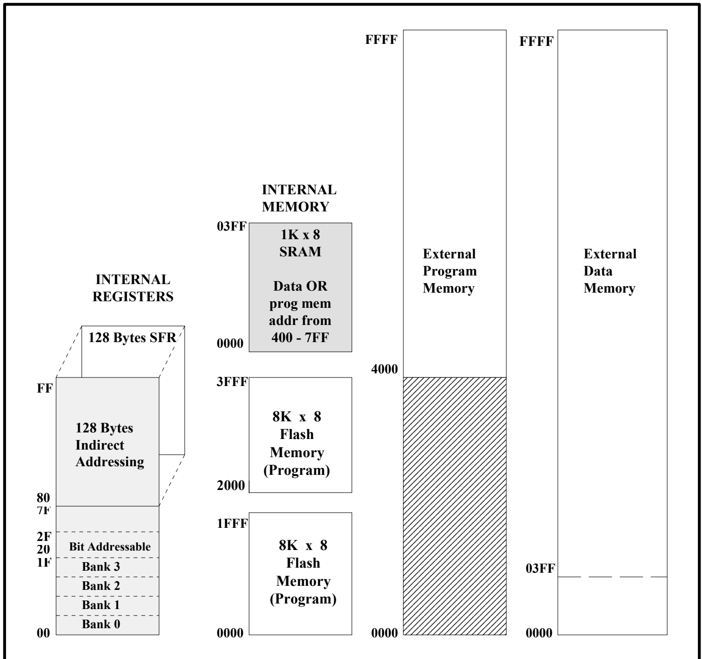
Figure 6. Memory Map
