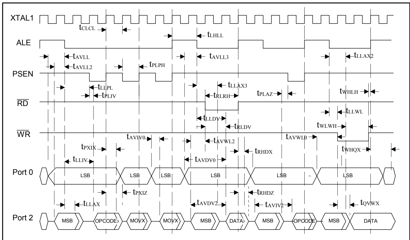
Figure 3. Page-Mode 2 Timing
