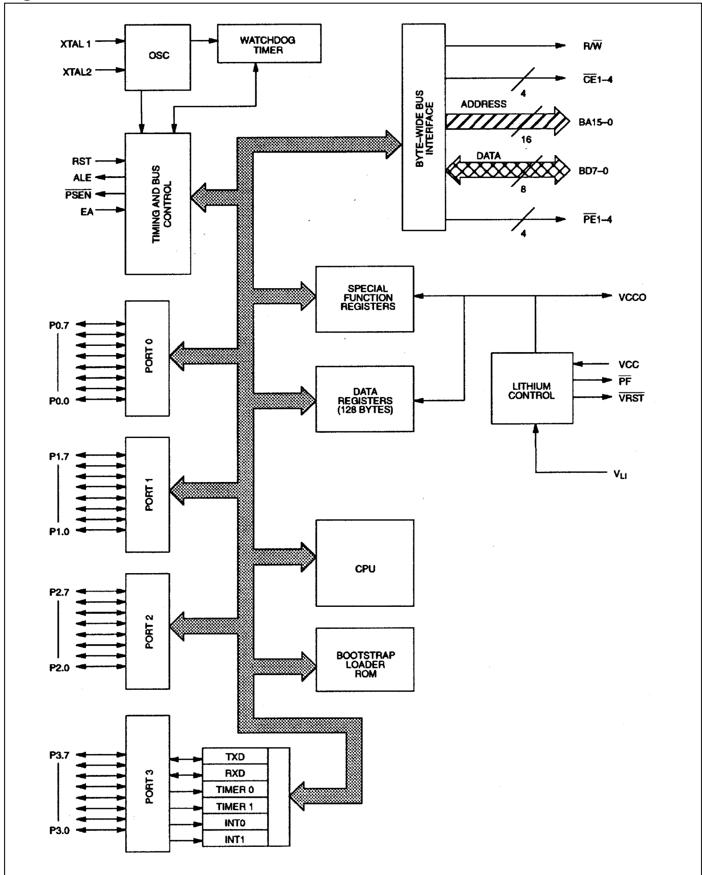
Figure 1. BLOCK DIAGRAM
