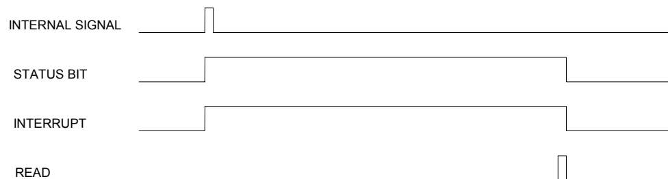
Figure 4.3A. EVENT STATUS BIT
