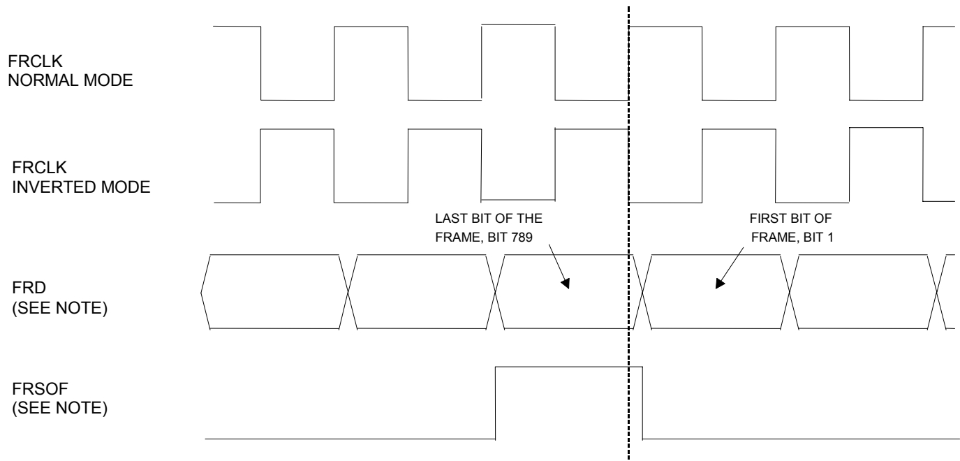
Figure 2.3B. RECEIVE FRAMER TIMING
