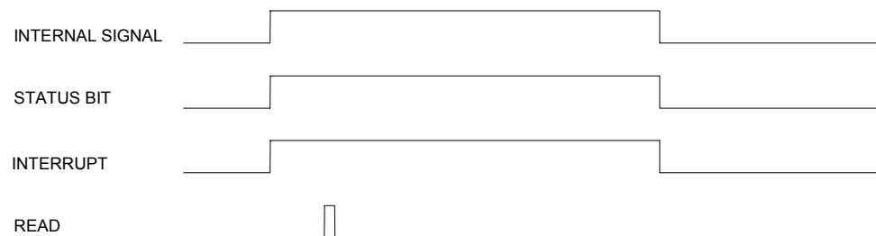
Figure 4.3C. REAL-TIME STATUS BIT
