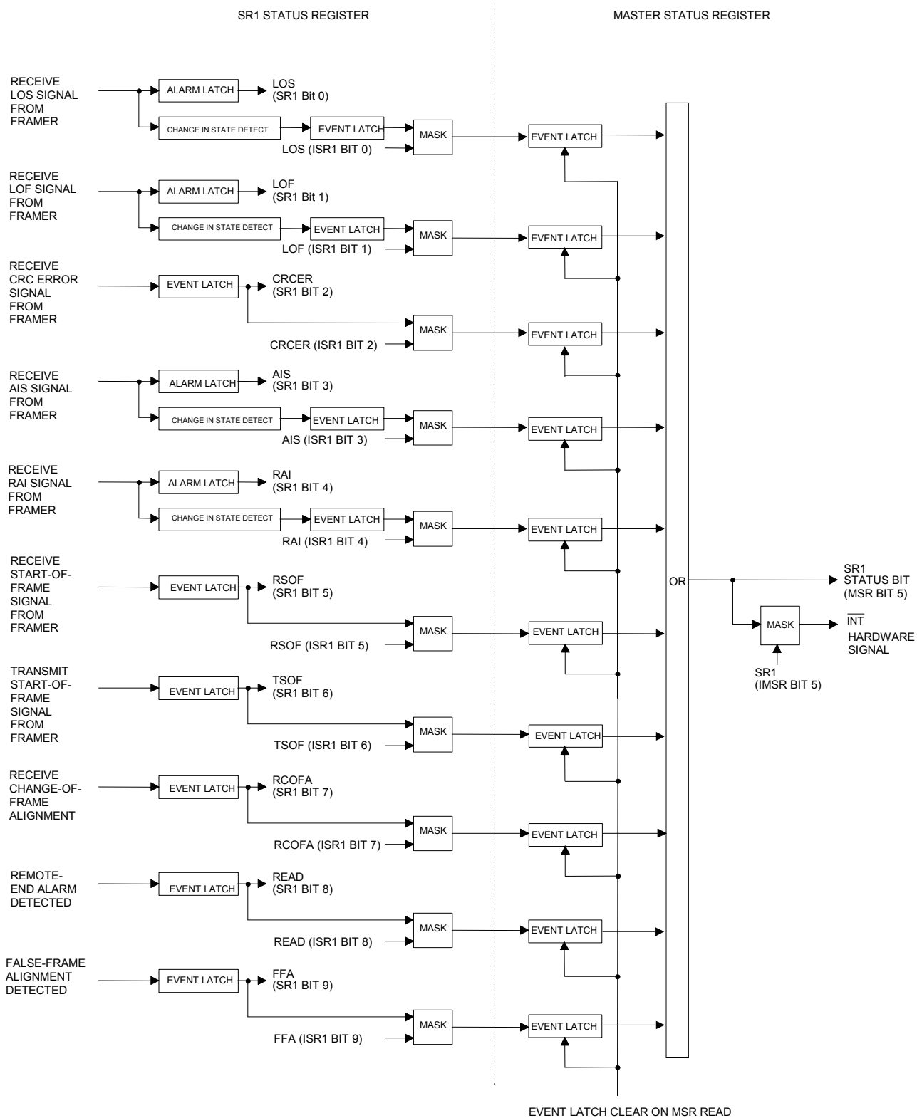
Figure 5.3A. SR1 STATUS BIT FLOW
