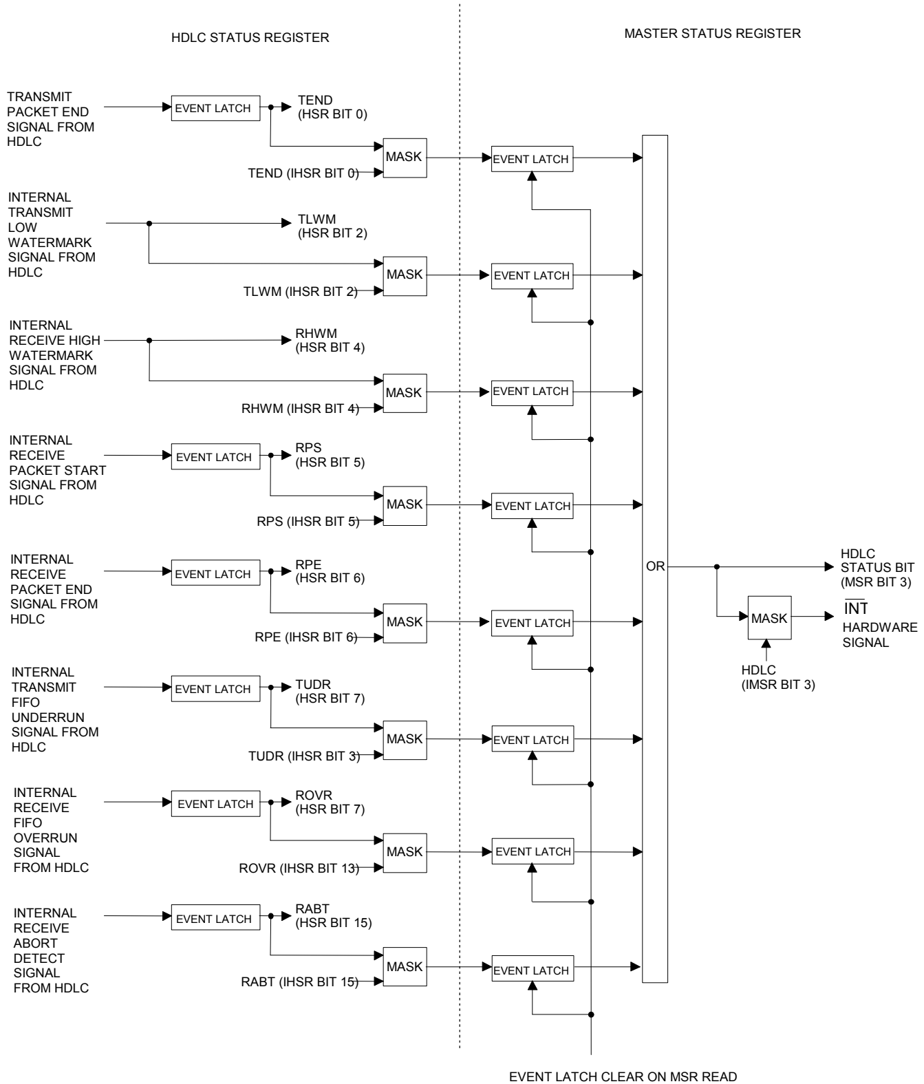
Figure 4.3E. HDLC STATUS BIT FLOW
