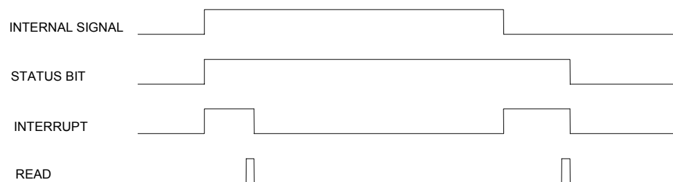
Figure 4.3B. ALARM STATUS BIT
