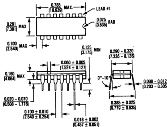
14 Lead Cerdip (JD) \theta_{JA} = 105^{\circ}\text{C/W} \theta_{JC} = 50^{\circ}\text{C/W}
