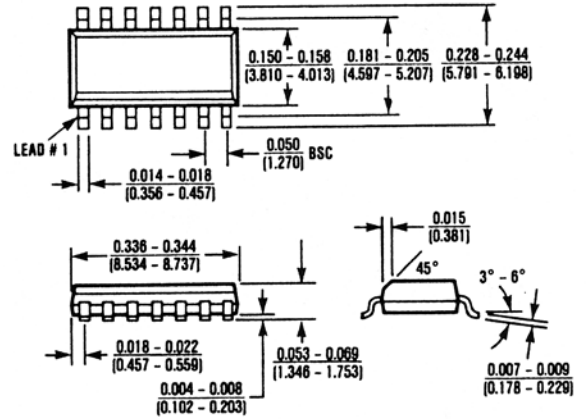
14 Lead Small Outline (SD) \theta_{JA} = 115^{\circ}\text{C/W} \theta_{JC} = 60^{\circ}\text{C/W}
