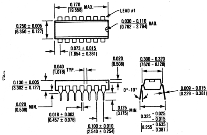
14 Lead Plastic DIP (PD) \theta_{JA} = 140^{\circ}\text{C/W} \theta_{JC} = 70^{\circ}\text{C/W}
