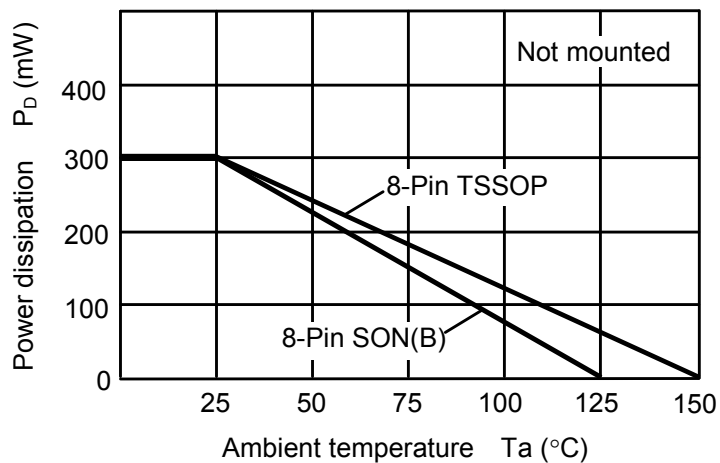
Figure 22 Power Dissipation
