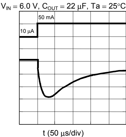
Figure 19 Ringing Waveform due to Load Variation (VOUT Pin)
