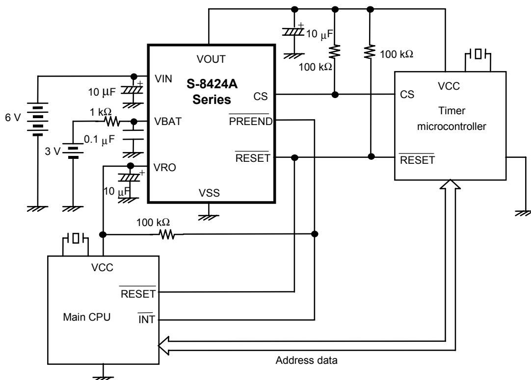
Figure 23 Application Circuit 1
