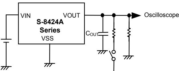
Figure 18 Test Circuit
