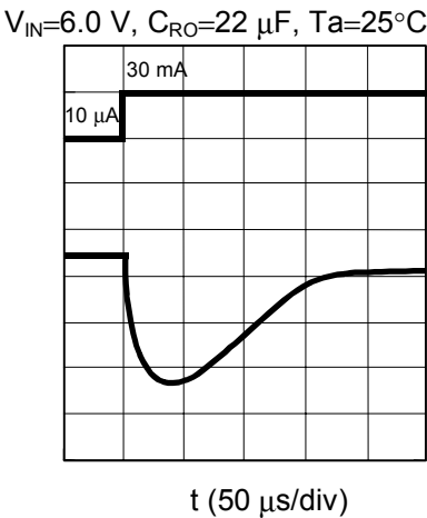
Figure 20 Ringing Waveform due to Load Variation (VRO Pin)
