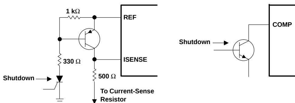
Figure 7. Shutdown Techniques
