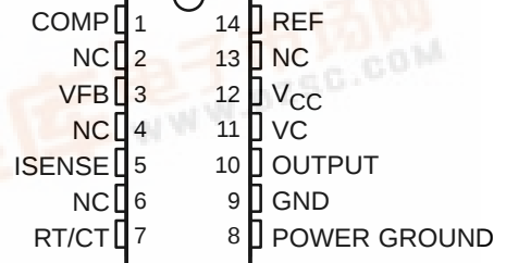
D PACKAGE (TOP VIEW)
