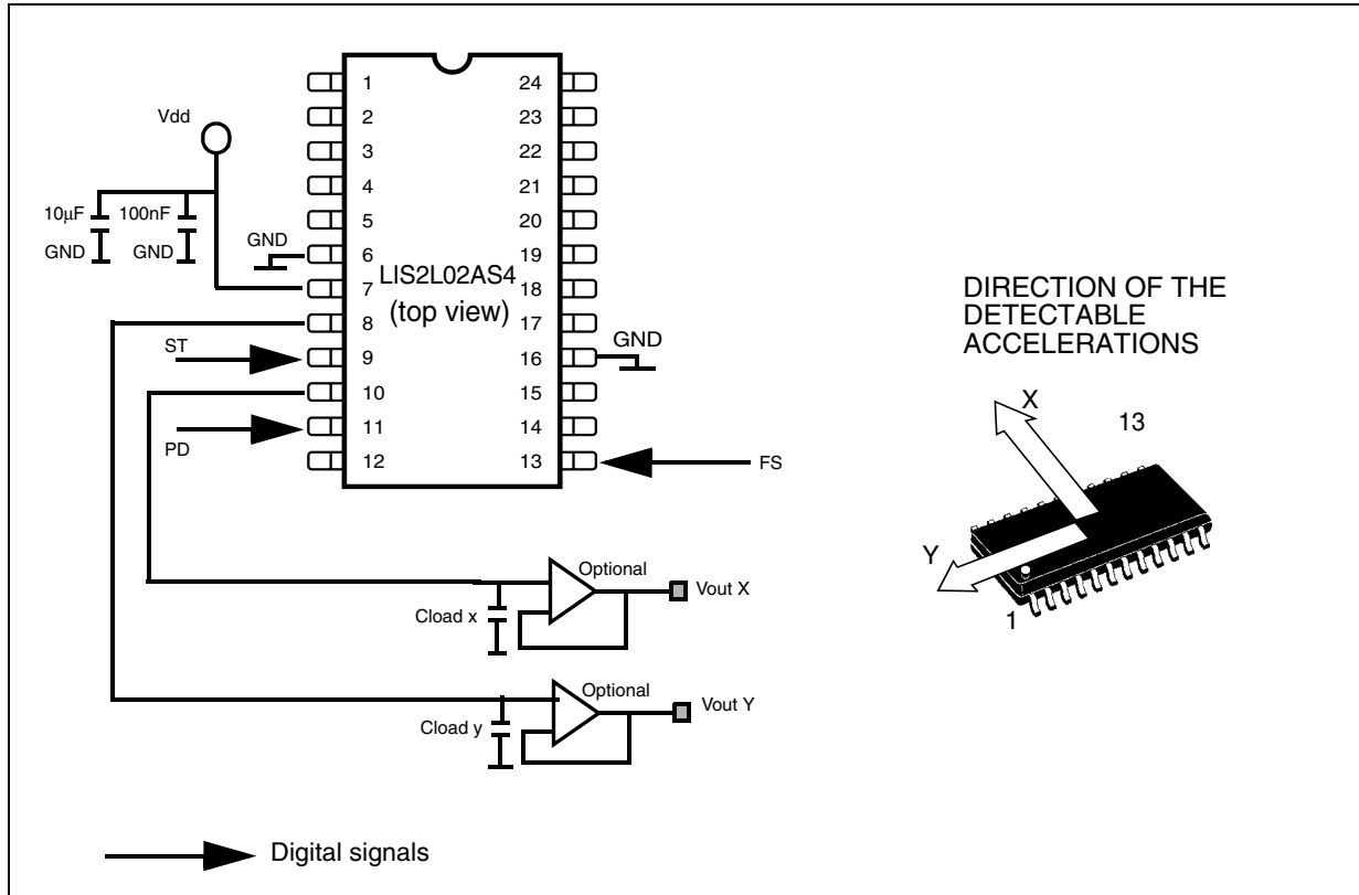
Figure 4. LIS2L02AS4 Electrical Connection
