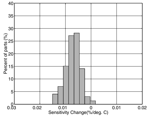
Figure 13. Y axis Sensitivity Change Vs. Temperature
