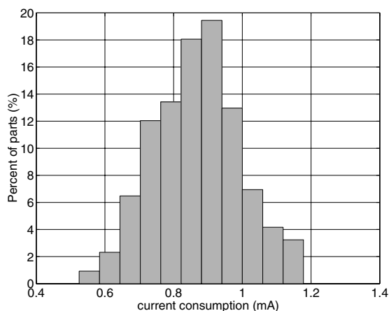
Figure 15. Current consumption at 3.3V
