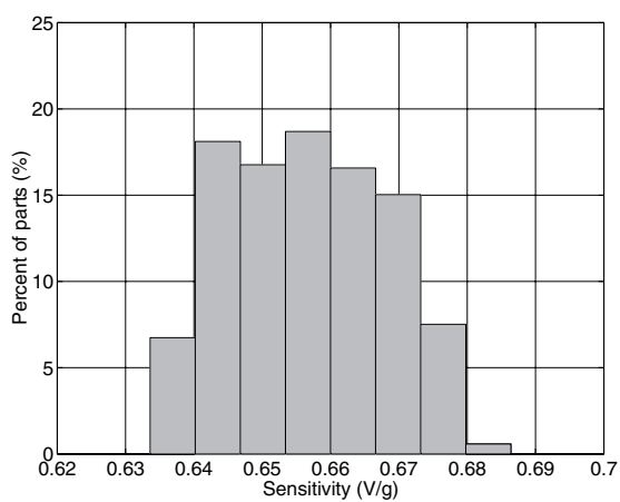
Figure 9. Y axis Sensitivity at 3.3V
