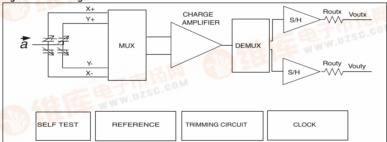
Figure 2. Block Diagram
