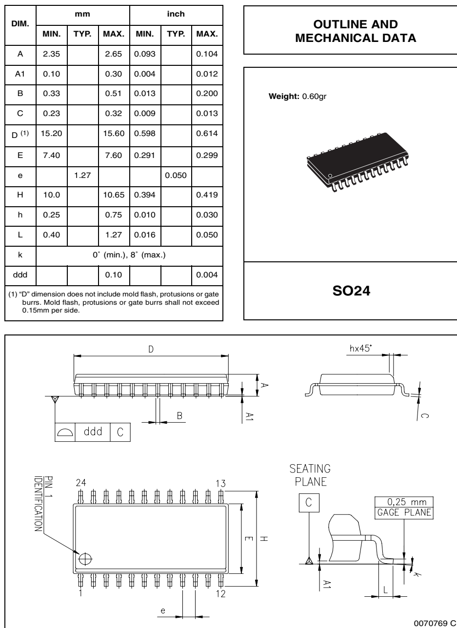
Figure 17. SO24 Mechanical Data & Package Dimensions
