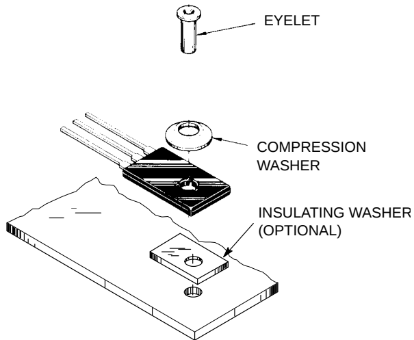
Figure 23. Eyelet Mounting
