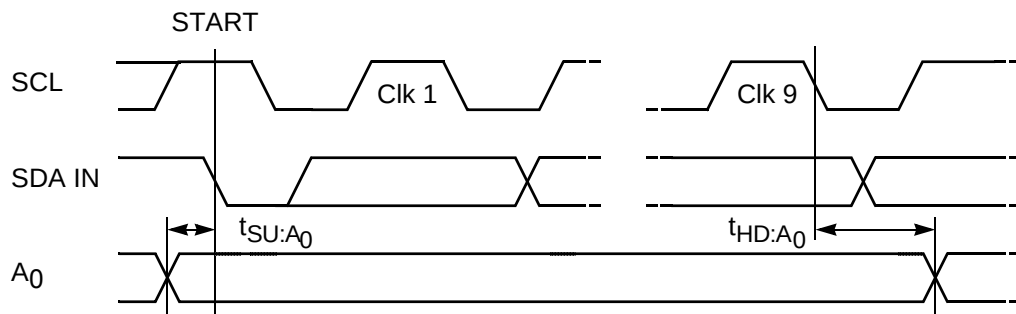
Figure 23. Physical Device Address ( A_0 ) Pin Timing
