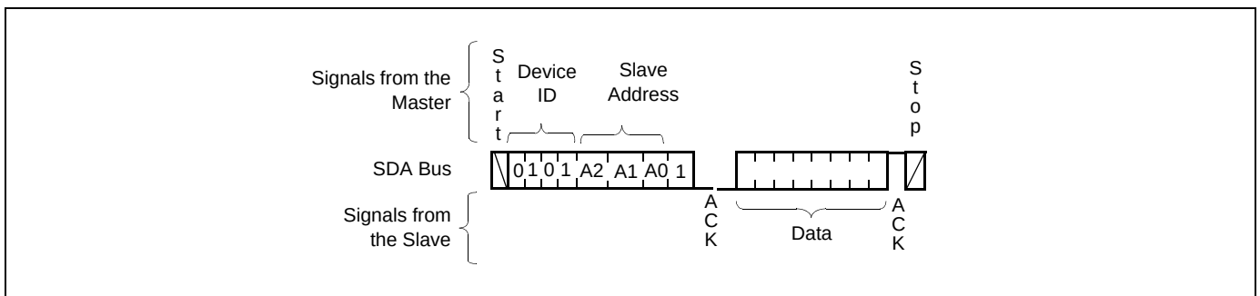
Figure 13. Current Address Read Sequence
