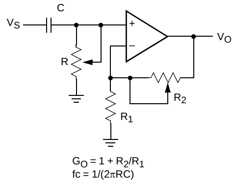
Filter
