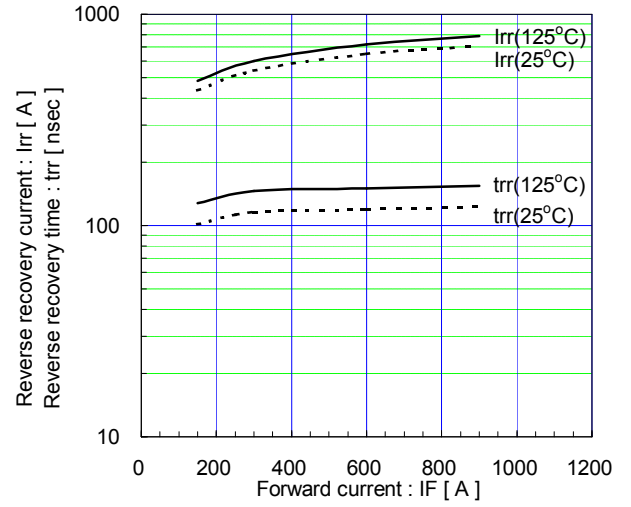
Reverse recovery characteristics (typ.) Vcc=600V, VGE=±15V, RG=1.1Ω
