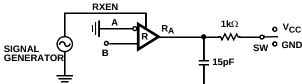
FIGURE 4. RS-485 RECEIVER PROPAGATION DELAY
