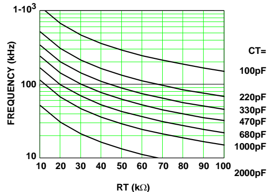
FIGURE 4. CAPACITANCE vs FREQUENCY
