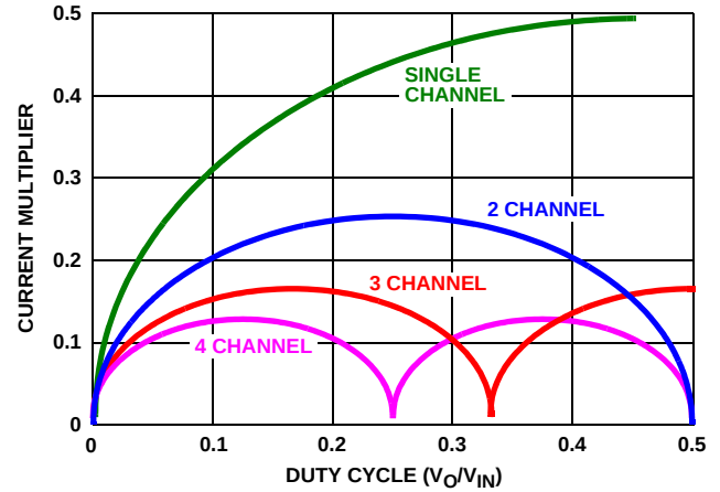
FIGURE 11. CURRENT MULTIPLIER vs DUTY CYCLE
