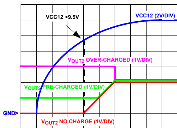
FIGURE 3. PRE-CHARGED OUTPUT
