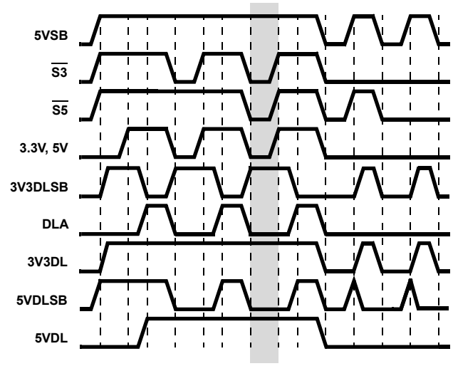
FIGURE 5. 5V_{DUAL} AND 3.3V_{DUAL}/3.3V_{SB} TIMING DIAGRAM; ISL6504A
