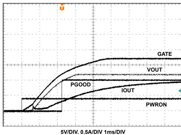
FIGURE 12. ISL6115 +12V TURN-ON
