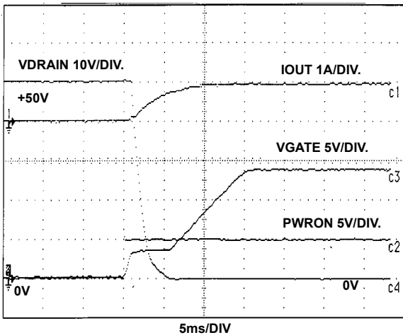
FIGURE 17. +50V LOW SIDE SWITCHING C_{GATE} = 100\text{pF}
