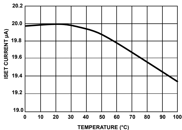
FIGURE 4. ISET SOURCE CURRENT
