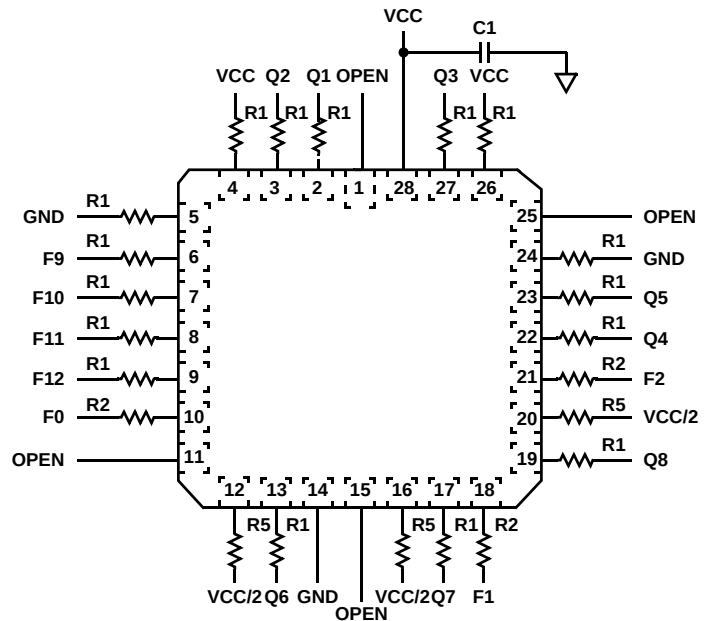
MR82C54 (CLCC)
