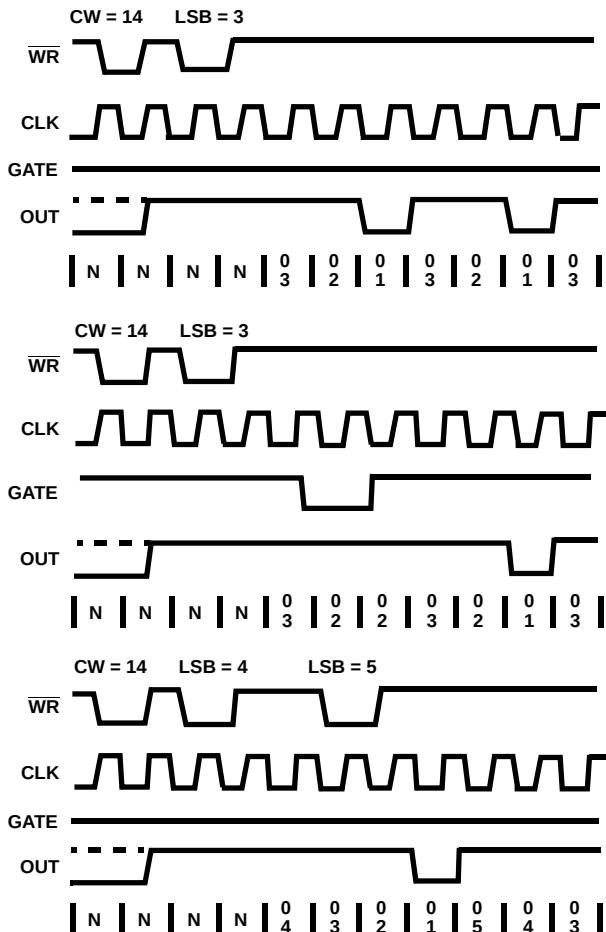
FIGURE 11. MODE 2
