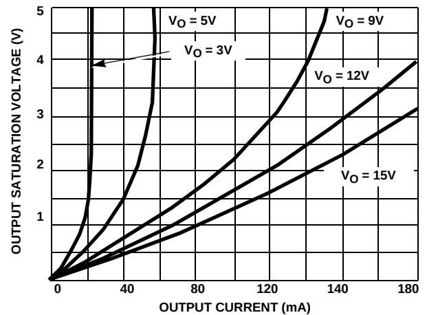
FIGURE 4. P_{\text{BAR}} OR S_{\text{BAR}} SATURATION VOLTAGE AS A FUNCTION OF OUTPUT CURRENT
