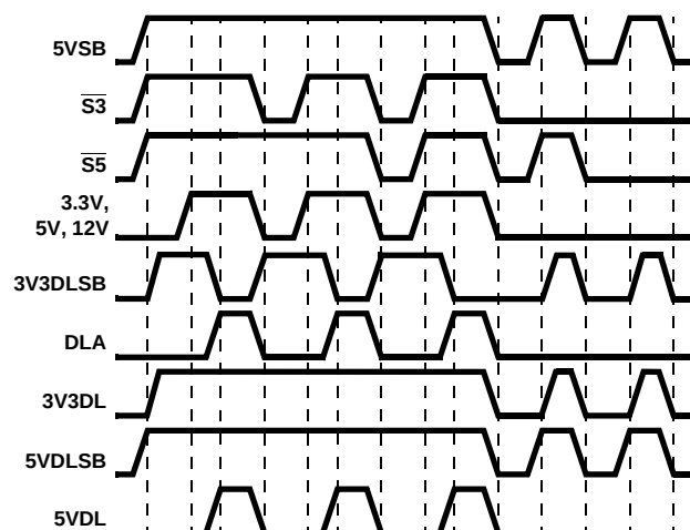
FIGURE 5. 5V_{DUAL} TIMING DIAGRAM FOR EN5VDL = 0 ; 3V_{DUAL}/3V_{SB}
