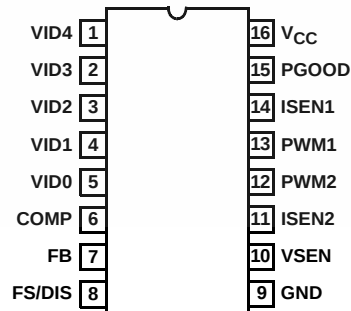
HIP6302 (SOIC) TOP VIEW
