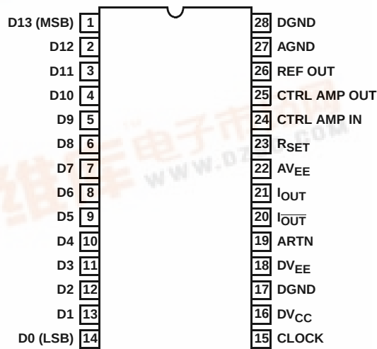
HI5741 (SOIC) TOP VIEW
