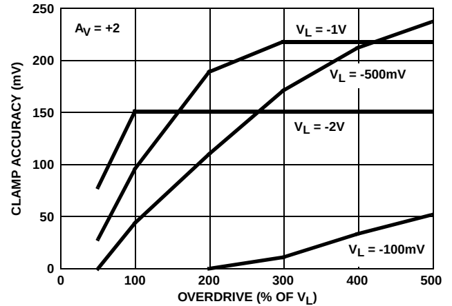
FIGURE 46. V_L CLAMP ACCURACY vs OVERDRIVE
