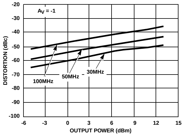
FIGURE 31. SECOND HARMONIC DISTORTION vs P_{\text{OUT}}
