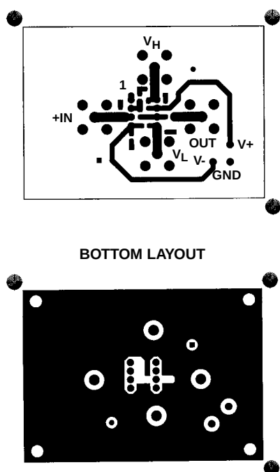
TOP LAYOUT
