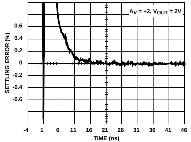
FIGURE 14. SETTLING RESPONSE
