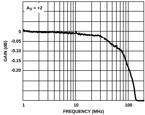
FIGURE 12. GAIN FLATNESS
