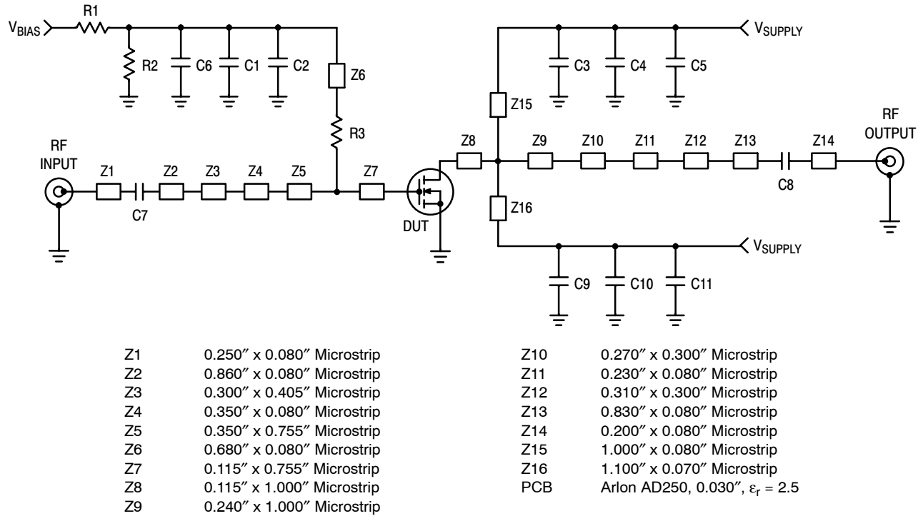
Figure 1. MRF6S21060NR1(NBR1) Test Circuit Schematic
