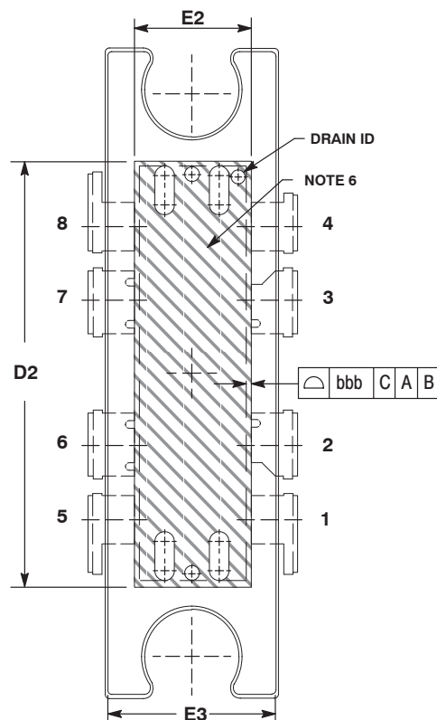
VIEW Y-Y
