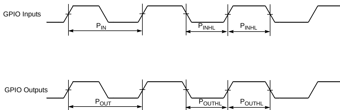
Figure 4-31 GPIO Timing
