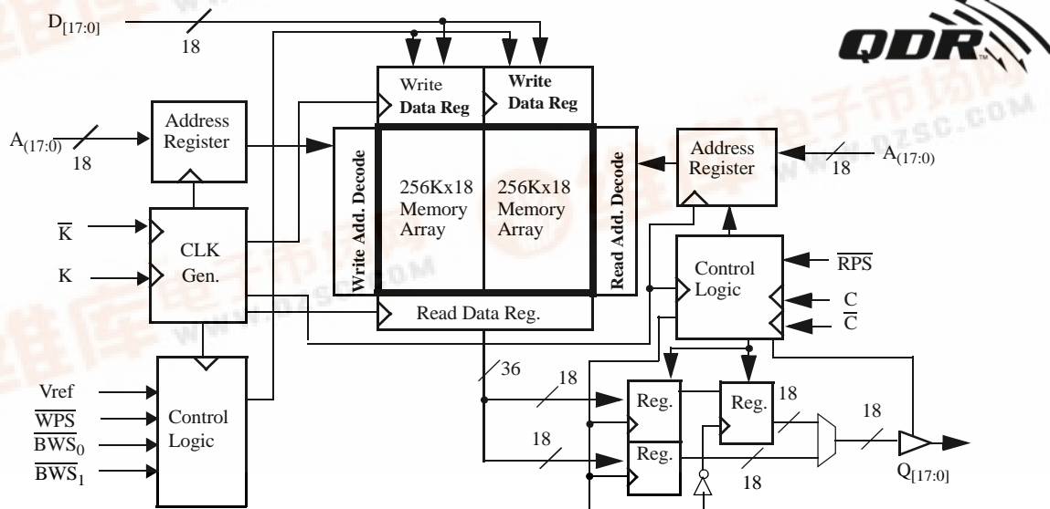
Logic Block Diagram (CY7C1302DV25)
