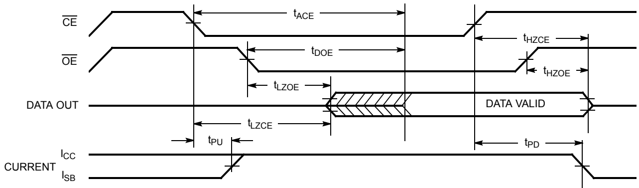
Read Cycle No. 3 (Either Port) [24, 26, 27, 28]
