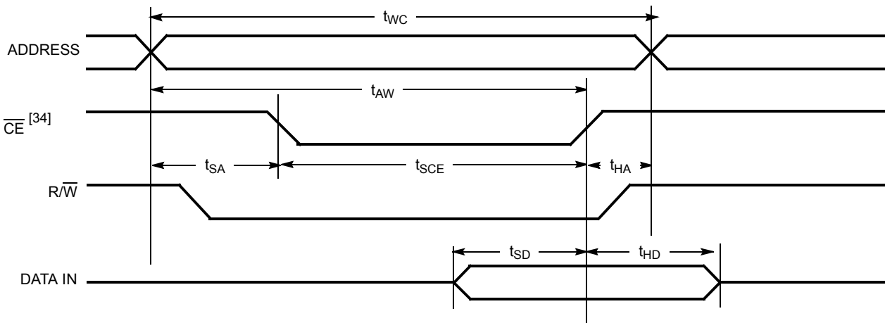
Write Cycle No. 2: CE Controlled Timing [29, 30, 31, 36]
