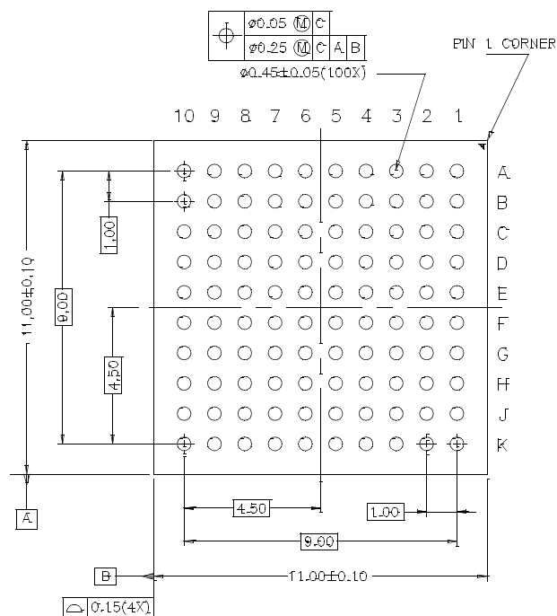
BOTTOM VIEW
