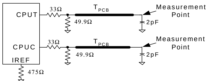
Figure 7.0.7V Load Configuration
