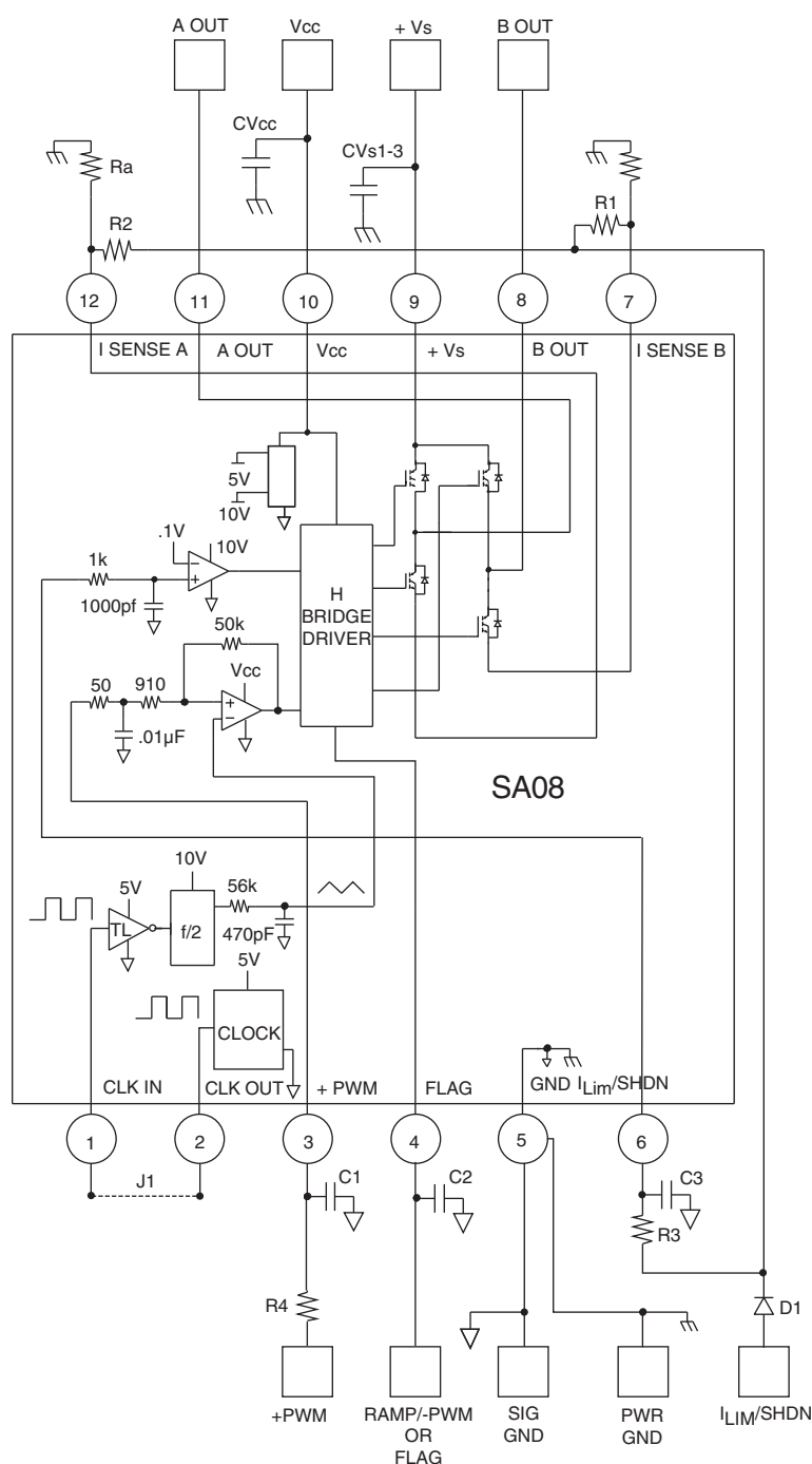
FIGURE 3. PCB SCHEMATIC.
