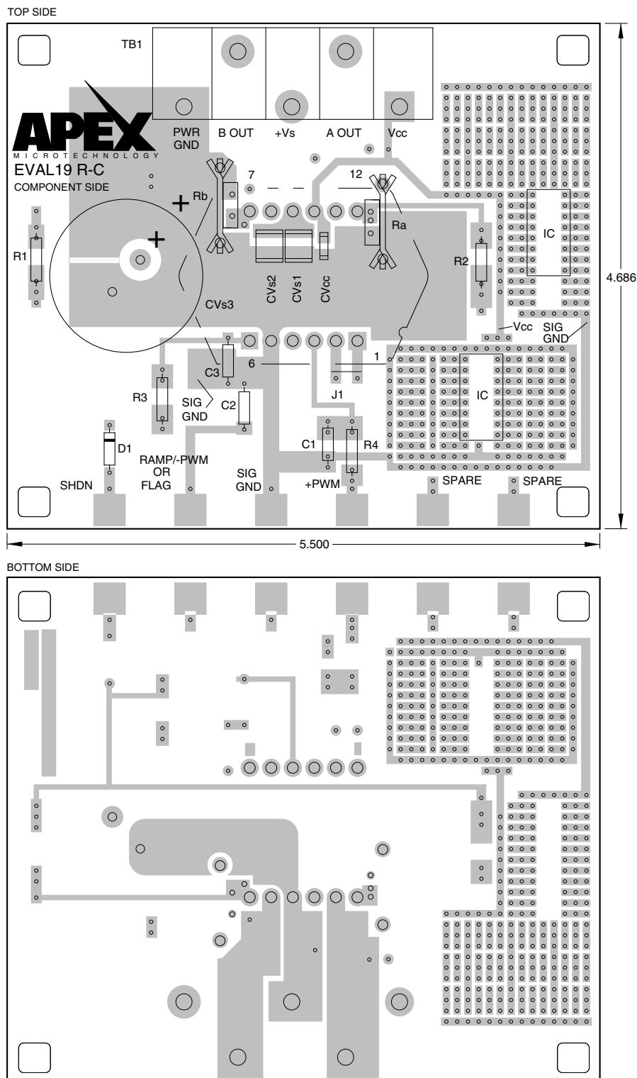
FIGURE 2. PCB
