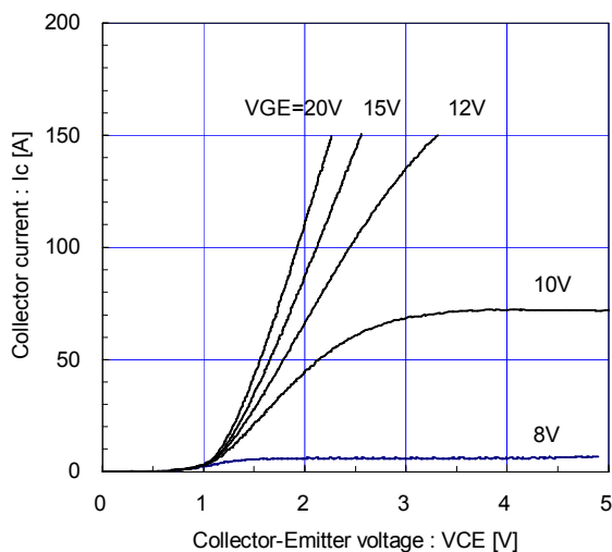
[ Inverter ] Collector current vs. Collector-Emittor voltage (typ.) T_j = 25^\circ\text{C} / chip
