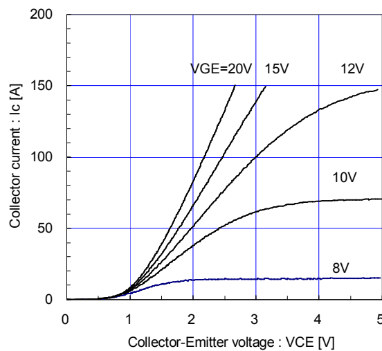
[ Inverter ] Collector current vs. Collector-Emittor voltage (typ.) T_j = 125^\circ\text{C} / chip
