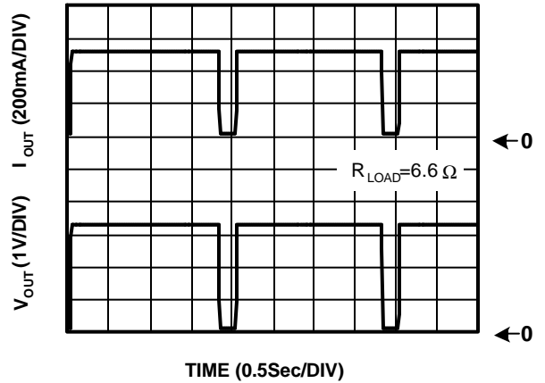
Overtemperature Shutdown
