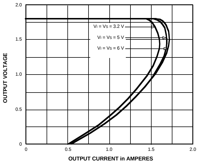
Overcurrent protection
