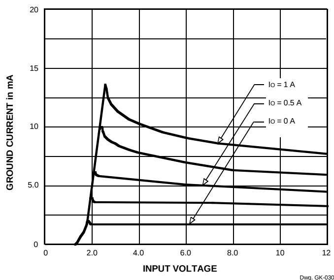
GND current
