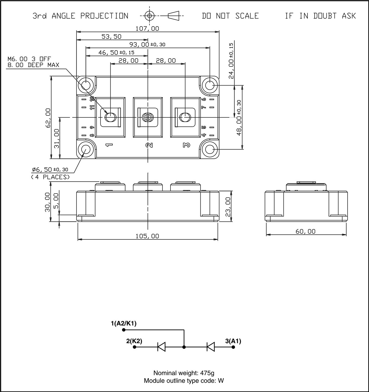
Fig. 8 Package details
