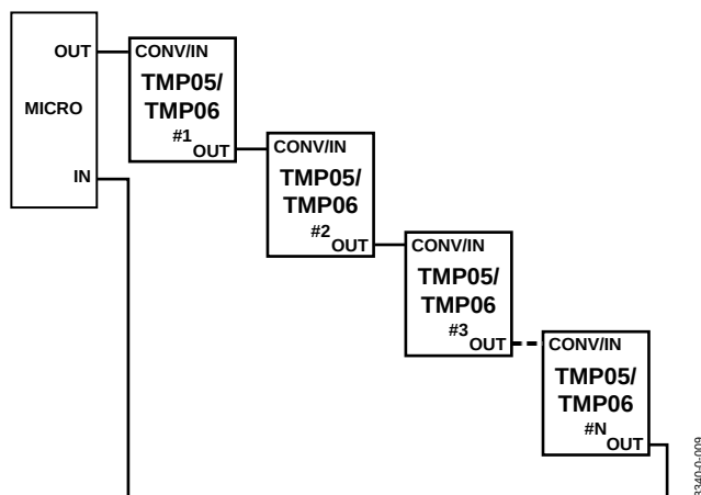
Figure 22. Daisy-Chain Structure
