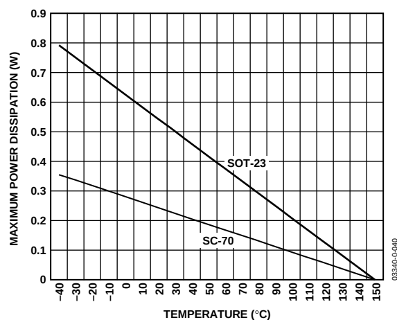
Figure 4. Maximum Power Dissipation vs. Temperature
