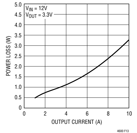
Figure 13. Power Loss vs Load Current
