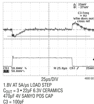
1.8V Transient Response
