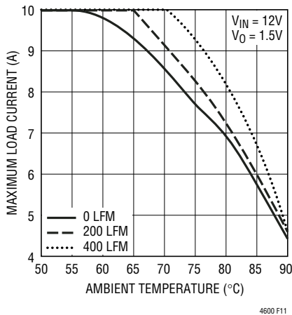
Figure 11. No Heatsink
