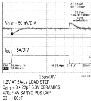
1.2V Transient Response
