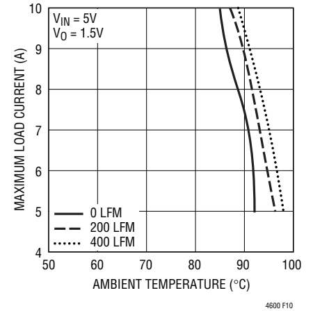
Figure 10. BGA Heatsink
