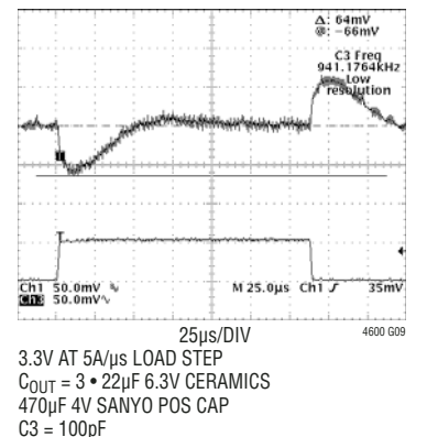
3.3V Transient Response
