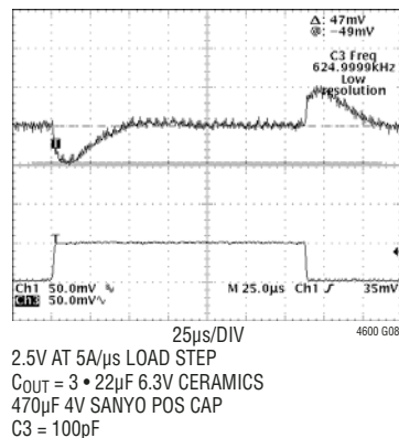
2.5V Transient Response
