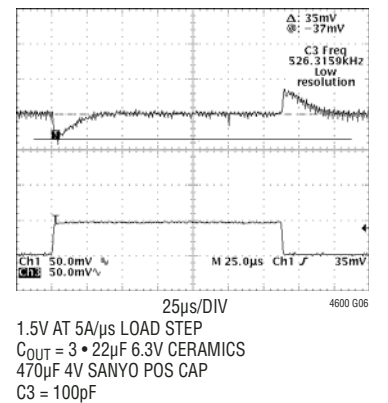
1.5V Transient Response
