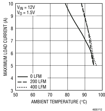
Figure 12. BGA Heatsink
