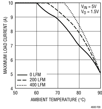
Figure 9. No Heatsink
